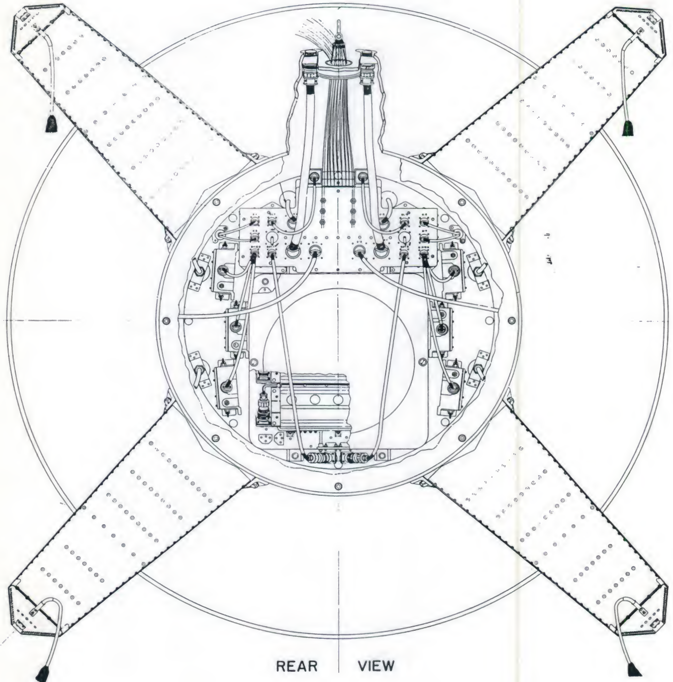
Fig. 5. -- Rear View of Mk IV Bomb
